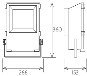
DELTA LED 85W / 100W
