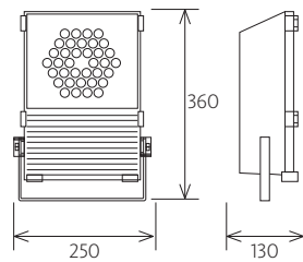
DELTA LED 35W
